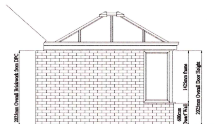
PROPOSED SOUTH ELEVATION
